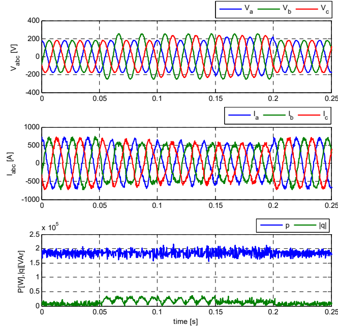
Fig. 10. Voltage, Current Grid and Active and Reactive Power injected during voltage swell.
