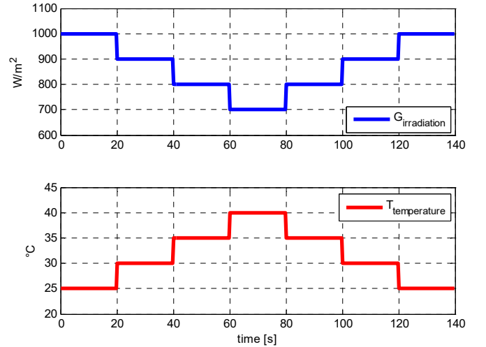
Fig. 5. Irradiation and Temperature Profile considered in the simulation results.
