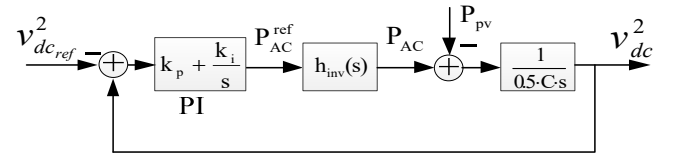
Fig. 4. DC link voltage control strategy.
