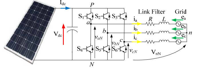
Fig. 2. Grid-connected photovoltaic system.
