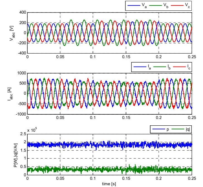
Fig. 11. Voltage, Current Grid and Active and Reactive Power injected during voltage swell.
