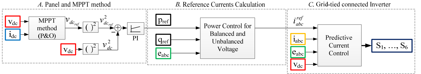
Fig. 3. Control Scheme for Grid-connected photovoltaic system for balanced and unbalanced grid voltage conditions.
